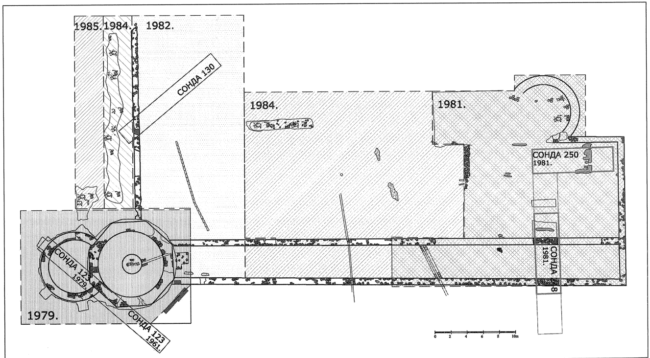
3. Mediana, villa with an octagon with areas explored during the excavations directed by Lj. Zotović (G. Milošević, according to the Documentation of the Archaeological Institute in Belgrade)
