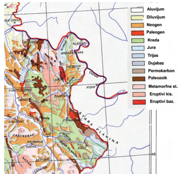
Fig. 2. Geological map of eastern Serbia
