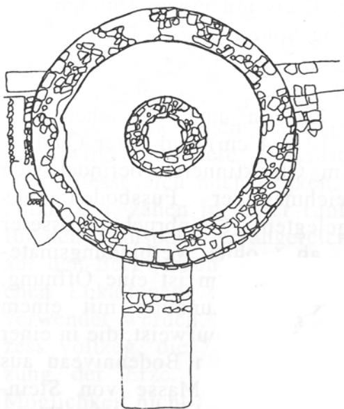
Fig. 15. Ground plan of circular structure 'for ore separation' in northeastern corner of Timacum Minus fortification
